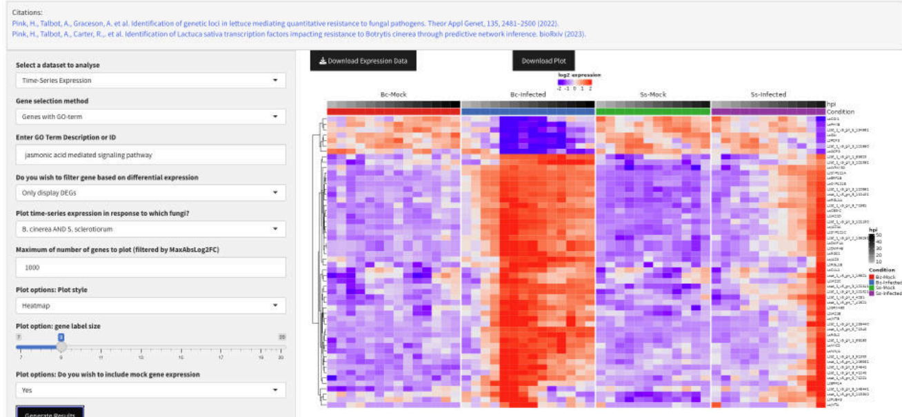
Figure C: An example output in the shiny app, where a user has selected a Heatmap displaying time-series expression for lettuce genes which are orthologues of Arabidopsis genes which are annotated with the GO-term “jasmonic acid mediated signalling pathway” (GO:0009867). The user has also selected to filter for just genes that are differentially expressed in the time-series. Download buttons above the plot enable the user to either download the plot or download the data used to produce the plot.
