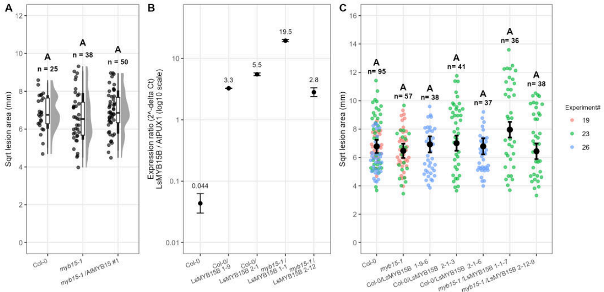
Figure 4.13: A) B. cinerea detached leaf assay of Col-0, myb15-1 and myb15-1/AtMYB15 #1 (generated by Chezem et al. 2017). Photos were taken of developing lesions at 72hpi, and measured with ImageJ. Raw data points, boxplots, and distribution of individual measured lesions are shown. Letters represent statistical significance groupings ( p < 0.05 ) B) delta Ct transgene expression ratio compared to an endogenous reference (AtPUX1) in Col-0/p35S::LsMYB15 and myb15-1 /p35S::LsMYB15. Tissue was collected from pooled samples of 10-day T 2 seedlings grown on 1/2 MS + BASTA plates. Col-0 seedlings were grown in parallel on 1/2 MS plates without BASTA. C) B. cinerea detached leaf assay susceptibility testing of LsMYB15 expressing transgenic Arabidopsis lines. Raw data values are shown by coloured points, with colour denoting the experimental replicate. Black points represent the predicted least-squares mean sqrt lesion area derived from a linear-mixed effect model (REML), with error bars indicating the REML standard error. Letters represent statistical significance groups ( p < 0.05 ) determined by a post-hoc Tukey HSD test performed on the REML model using lmerTest and predictmeans R packages. 'n' represents the total number of individual lesions measured across all experiments.
