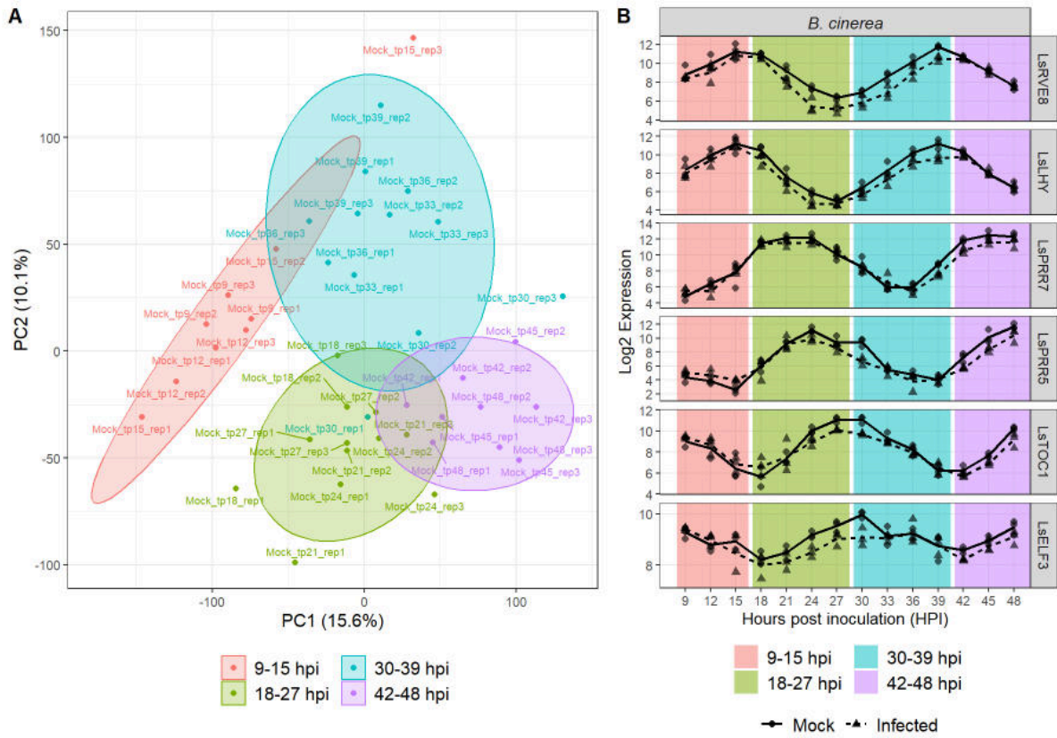
Figure 3.3: Circadian Oscillation observed in Lettuce time-series. (A) Principal Component Analysis of mock inoculated gene expression, PC1 is plotted on the x axis, PC2 is plotted on the y axis accounting for 15.6% and 10.1 % of variation respectively. Samples between 9 and 15 hours post inoculation (hpi) are coloured in red, 18 to 27 hpi samples are green, 30 to 39 hpi in blue and 42 to 48 hpi. (B) Expression of circadian regulators in lettuce time-series, mock expression shown by circles and solid lines B. cinerea infected expression shown by triangles and dotted lines. LsRVE8 ( Lsat_1.v5_gn.2.109801 ), LsLHY ( Lsat_1.v5_gn.3.140720 ), LsPRR5 ( Lsat_1.v5_gn.8.4341 ), LsPRR7 ( Lsat_1.v5_gn.2.115441 ), LsTOC1 ( Lsat_1.v5_gn.1.14320 ) and LsELF3 ( Lsat_1.v5_gn.6.7561 ).
