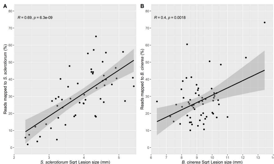
Figure 2.7: Pearson's correlation of RNAseq reads in each sample that map to fungal transcripts versus lesion size in (A) S. sclerotiorum and (B) B. cinerea inoculated samples.
