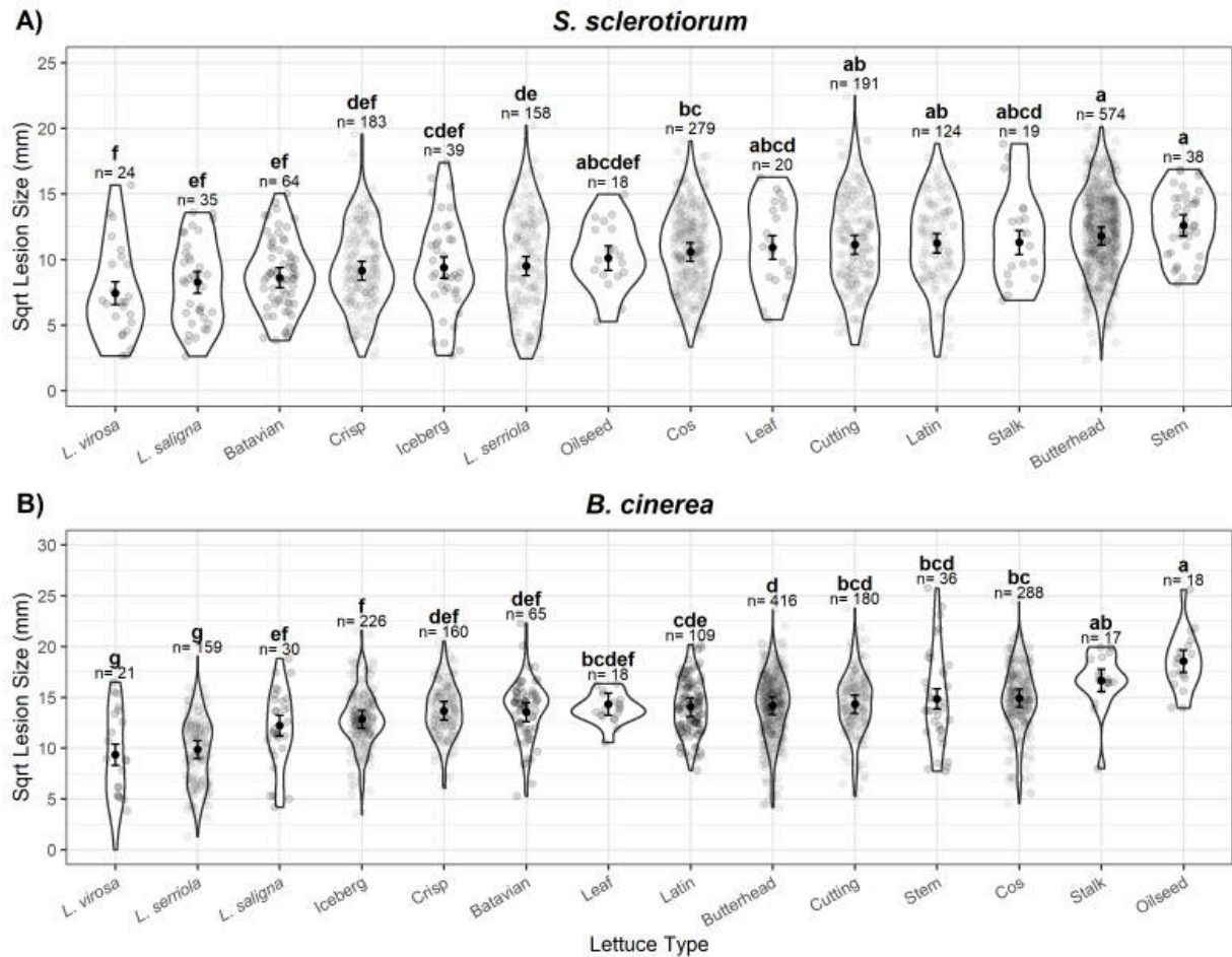
Figure 2.2: Variation in lesion size after inoculation with B. cinerea or S. sclerotiorum between lettuce types. Square root lesion size in response to S. sclerotiorum (top) or B. cinerea (bottom) on detached lettuce leaves of the Lettuce Diversity Fixed Foundation Set. Grey points show individual measured lesions, violins show the distribution. Black points show REML predicted (accounting for random variation between experimental replicates). Error bars indicate REML predicted standard error. Letters shown represent Tukey HSD significance groupings ( p < 0.05 ). n = the number of lesions measured from each type in response to each pathogen.
