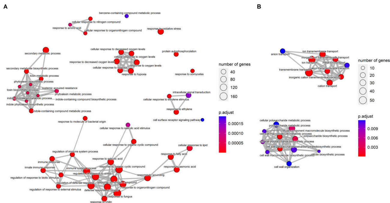
Figure 4.4: LsERF1 OE2-mock vs WT-mock GO-enrichment network plot. Network edges represent GO-terms containing \geq 33\% overlapping Arabidopsis orthologues of DEGs. The size of the node represents the number of unique Arabidopsis orthologues of DEGs. Colour represents the statistical significance, of the enrichment, with red nodes showing higher significance. A) GO-enrich network for upregulated DEGs, B) GO-enrich network for downregulated DEGs
