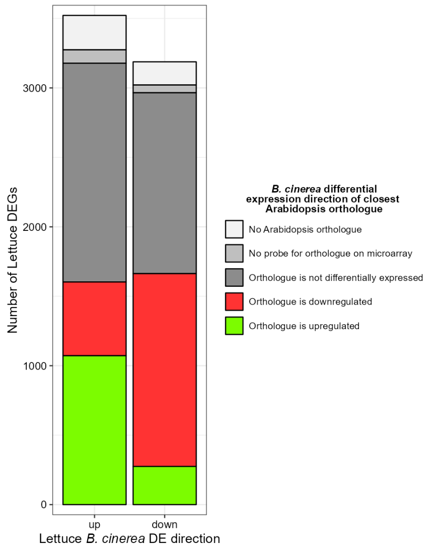
Figure 3.6: Species specificity of transcriptional reprogramming during B. cinerea infection. Bar chart showing the number of lettuce genes up and downregulated after inoculation with B. cinerea . Bars are coloured by the direction of differential expression following B. cinerea inoculation of the single closest Arabidopsis orthologue for each lettuce DEG (Windram et al. 2012). Orthologues were as described in Reyes-Chin-Wo et al. 2017.
