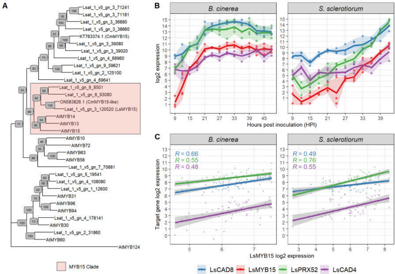
Figure 4.12: A ) 2000-bootstrap maximum likelihood phylogenetic tree containing Arabidopsis R2-R3 MYB subgroups 1-3, their putative lettuce orthologues, Chrysanthemum MYB15 orthologues and AtMYB124 as an outgroup. B ) Expression of Lsat_1_v5_gn_3_120520 (LsMYB15 - red), Lsat_1_v5_gn_9_111281 (LsCAD4 - purple), Lsat_1_v5_gn_2_69560 (LsCAD8 - blue) and Lsat_1_v5_gn_5_175321 (LsPRX52 - green) after B. cinerea (left panel) and S. sclerotiorum (right panel) infection, mock-expression not shown. Hours post inoculation on X-axis, log 2 expression on Y-axis. Points show individual biological replicates, line is drawn through time-point mean, shaded area shows the 95% confidence interval. C ) Lettuce diversity-panel co-expression (data from Pink et al. 2022), LsMYB15 log 2 expression is shown on X-axis, log 2 expression of putative target genes is shown on Y-axis (same genes and colours as Panel B). Expression after B. cinerea infection on left panel, and expression after S. sclerotiorum infection on right panel. Pearson's correlation coefficient for gene expression shown, with colour denoting which target gene the co-expression refers to.
