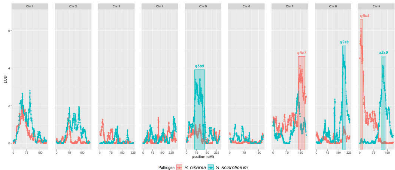
Figure 2.14: Quantitative trait loci associated with reduced lesion size of B. cinerea or S. sclerotiorum . LOD scores from 'stepwiseqtl' multi-QTL selection models using the Haley-Knott algorithm, genotyping-by-sequencing markers and predicted mean lesion size from the detached leaf assay data for each pathogen are shown. Data relating to B. cinerea inoculation are shown in red, whereas those from S. sclerotiorum inoculation are shown in blue. Five significant QTL ( qSs5 , qSs8 , qSs9 , qBc7 and qBc9 ) were maintained in the final model after backwards elimination of insignificant loci. Boxes represent the 1.5 LOD confidence intervals around the peak LOD of each QTL. The nine lettuce chromosomes are shown along the x-axis.
