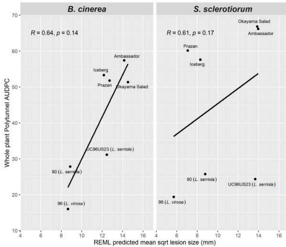
Figure 2.6: Correlation of REML predicted detached leaf assay square root lesion size (mm) with AUDPC in whole plant inoculations of B. cinerea (left) and S. sclerotiorum (right) for seven lettuce accessions. Pearson's correlation coefficient ( R ) values and p -values are shown. All accessions are L. sativa unless otherwise indicated.
