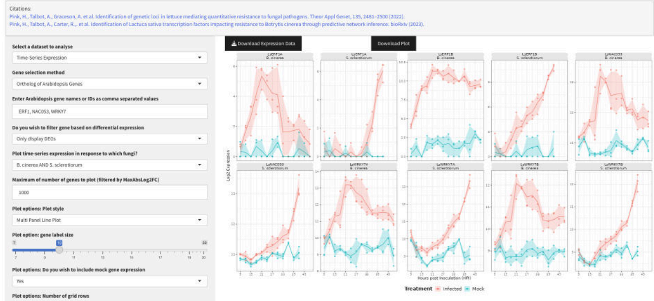
Figure B: An example output in the Shiny App, where a user has selected a “Multi Panel Line Plot” of Time-Series Expression for lettuce orthologues of “ERF1, NAC053, WRKY7” with filters applied to only display genes differentially expressed in the time-series. Download buttons above the plot enable the user to either download the plot or download the data used to produce the plot.
