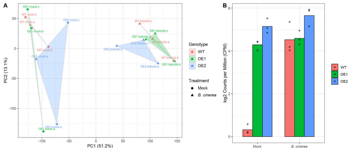
Figure 4.2: (A) Principal Component Analysis (PCA) plot of log2 counts per million (log2 CPM) expression at a gene-level. Circles represent mock samples, triangles represent B. cinerea infected samples. Point colour denotes the genotype of the sample; red = wt-sib (107-6), green = OE1 (107-7) and blue = OE2(148-9). (B) Log2 CPM expression of LSATv11_C03_021665 (LsERF1).
