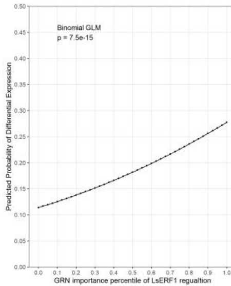
Figure 4.6: Model-predicted probability of a given gene being identified as a differentially expressed gene (DEG) in p35S::LsERF1 transgenic lines based on GRN importance score of its interaction with LsERF1. X-axis represents the importance score percentile of the predicted regulation by LsERF1. Y-axis shows the GLM predicted probability of a gene being differentially expressed. Points show GLM predictions made at specific percentile values.
