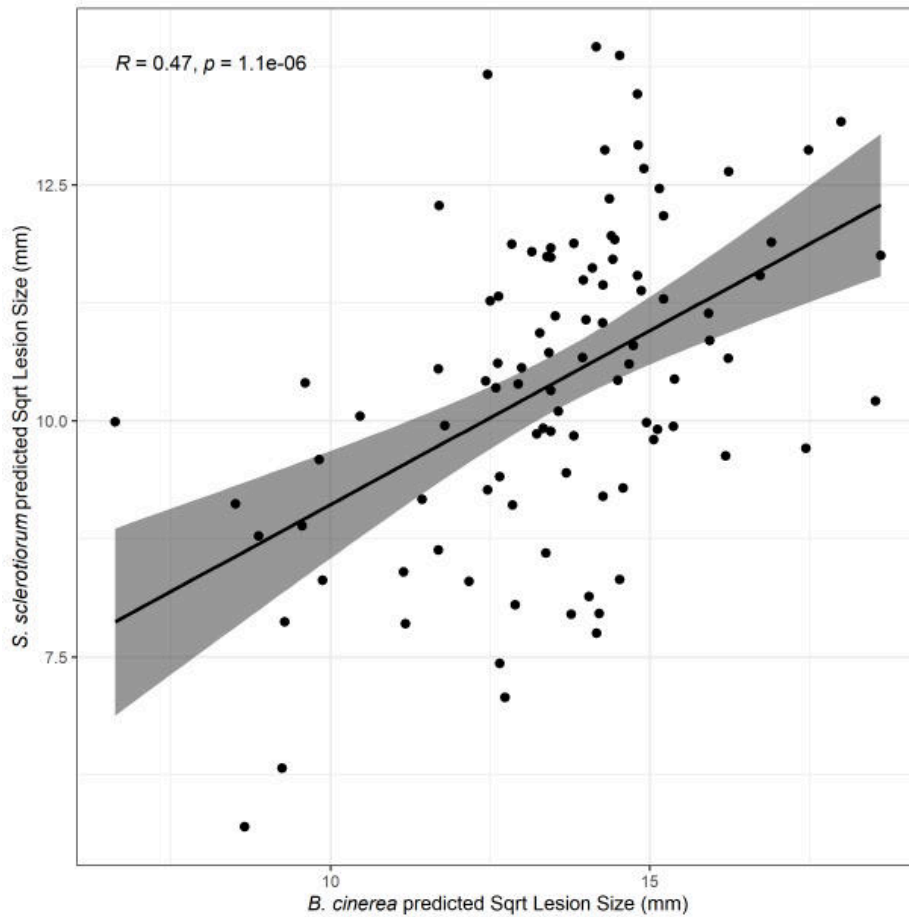
Figure 2.4: Correlation between lesion size 64 hours post inoculation with S. sclerotiorum and B. cinerea . Least-squares predicted mean square root lesion size of B. cinerea (x-axis) vs. S. sclerotiorum (y-axis) on detached lettuce leaves, where n ranges from two to 20 for each accession/pathogen combination. Linear regression line is shown in black, with 95% confidence intervals shaded in grey.
