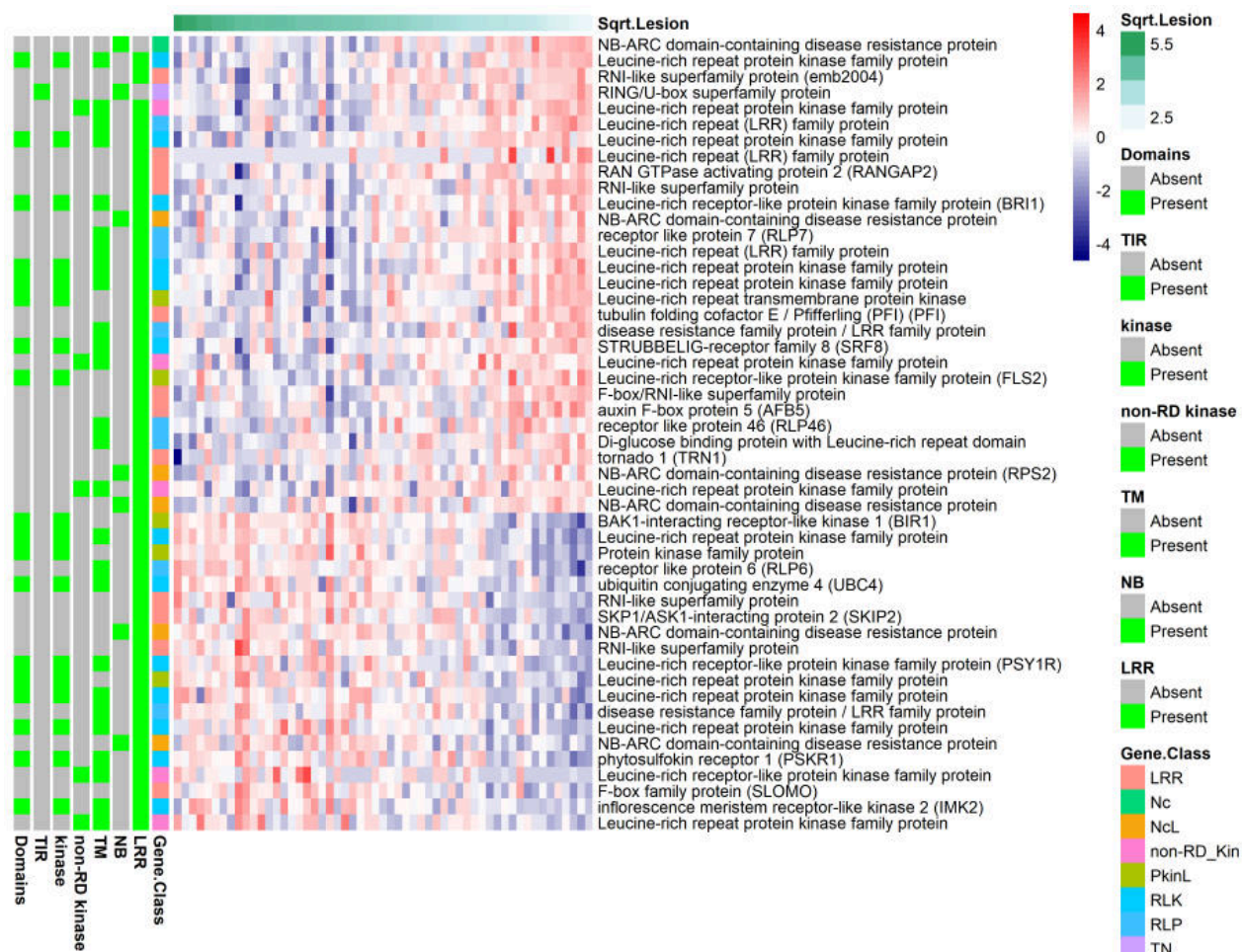
Figure 2.12: Expression of the top 50 lettuce genes whose expression is correlated with S. sclerotiorum lesion size, and which were classified as non-NLR pathogen recognition receptors (Christopoulou et al. 2015) classification indicated in the column gene.class). This classification was based on the presence of any combination of the following domains; leucine-rich repeats (LRR), nucleotide-binding (NB), NB Coiled-coil type (Nc), transmembrane (TM), kinase, non-arginine-aspartate kinase (non-RD kinase) and TOLL/interleukin-1 receptor (TIR). Additional gene nomenclature includes NcL: NC plus L domains; PkinL: kinase plus L; RLK: receptor-like kinase; RLP receptor-like protein. The individual lettuce samples are ordered left to right on the basis of lesion size after inoculation with S. sclerotiorum , with the most susceptible (largest lesion size) on the left and most resistant (smallest lesion size) on the right. Log2 expression is indicated by the red/blue scale
