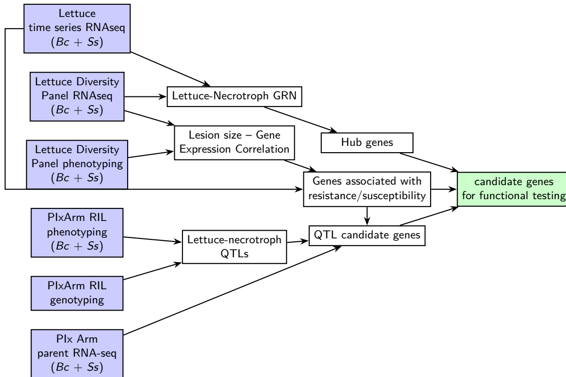
Figure 5.1: Flow diagram of the integrative analysis to identify candidate genes in lettuce for necrotrophic pathogen resistance. Input datasets are listed on the left; Lettuce-necrotroph time series RNAseq : high-density time series gene expression data during B. cinerea ( Bc ) or S. sclerotiorum ( Ss ) infection (Pink et al. 2023; Ransom et al. 2023); Lettuce Diversity Panel RNAseq : gene expression after B. cinerea and S. sclerotiorum infection in 21 diverse lettuce accessions (Pink et al. 2022); Lettuce Diversity Panel necrotroph phenotyping : quantitative detached leaf assay phenotyping of B. cinerea and S. sclerotiorum resistance in diverse lettuce accessions (Pink et al. 2022); PI x Arm RIL necrotroph phenotyping : quantitative detached leaf assay phenotyping of B. cinerea and S. sclerotiorum resistance in 236 F 6 recombinant inbred lines (RILs) from the PI251246 x Armenian L. serriola mapping population (PlxArm) (Pink et al. 2022); PI x Arm RIL genotyping : 2677 markers for the PlxArm population were previously described by Han et al. 2021; PlxArm parent RNA-seq : gene expression in mapping population parents PI251246 and Armenian L. serriola (Pink et al. 2022).
