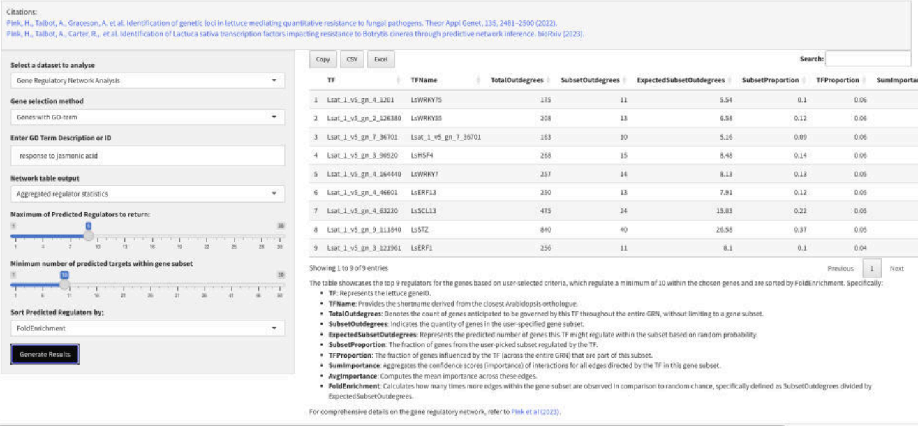
Figure D: An example output in the shiny app, identifying predicted gene regulatory network hubs for specific genes of interest. The user has selected to view “Aggregated regulator statistics” for the transcription factors which are predicted to regulate lettuce orthologues of genes annotated with the GO-term “response to jasmonic acid”. The user has applied an additional filter, requiring the transcription factor to have at least 10 predicted targets within the subset to be listed, and the results have been ordered by “FoldEnrichment”.
