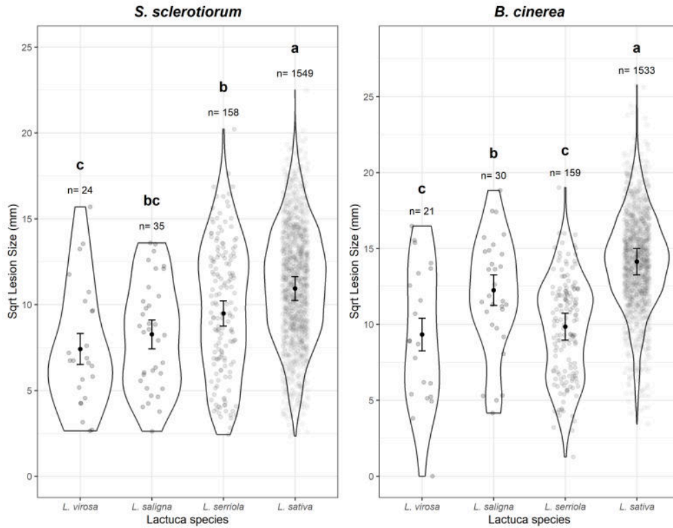
Figure 2.3: Variation in lesion size after inoculation with Botrytis cinerea or Sclerotinia sclerotiorum in different lettuce species. Square root lesion size 64 h after Sclerotinia sclerotiorum (left) or Botrytis cinerea (right) inoculation of detached lettuce leaves is shown. Grey circles represent individual measured lesions, with areas within the lines showing the distribution of data points. Black circles are the REML predicted mean lesion size per species (correcting for random variation between experimental replicates) with error bars showing REML predicted standard error. Letters represent Tukey post-hoc significance groupings ( p < 0.05 ) performed on the REML model. n is the number of lesions measured from each species.
